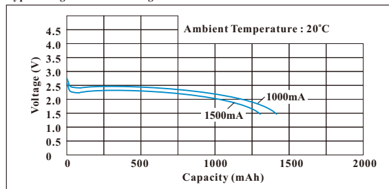
Typical High Drain Discharge Characteristics
